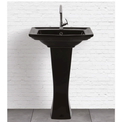
SOFIA-BLACK(Glossy) L 575 W 420 H 850 Weight - 23Kg.
